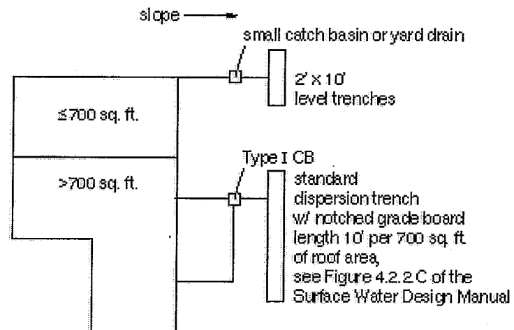
PLAN VIEW OF ROOF NTS
