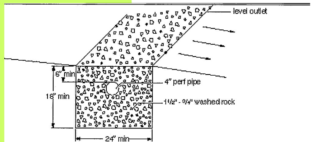
TRENCH X-SECTION NTS
