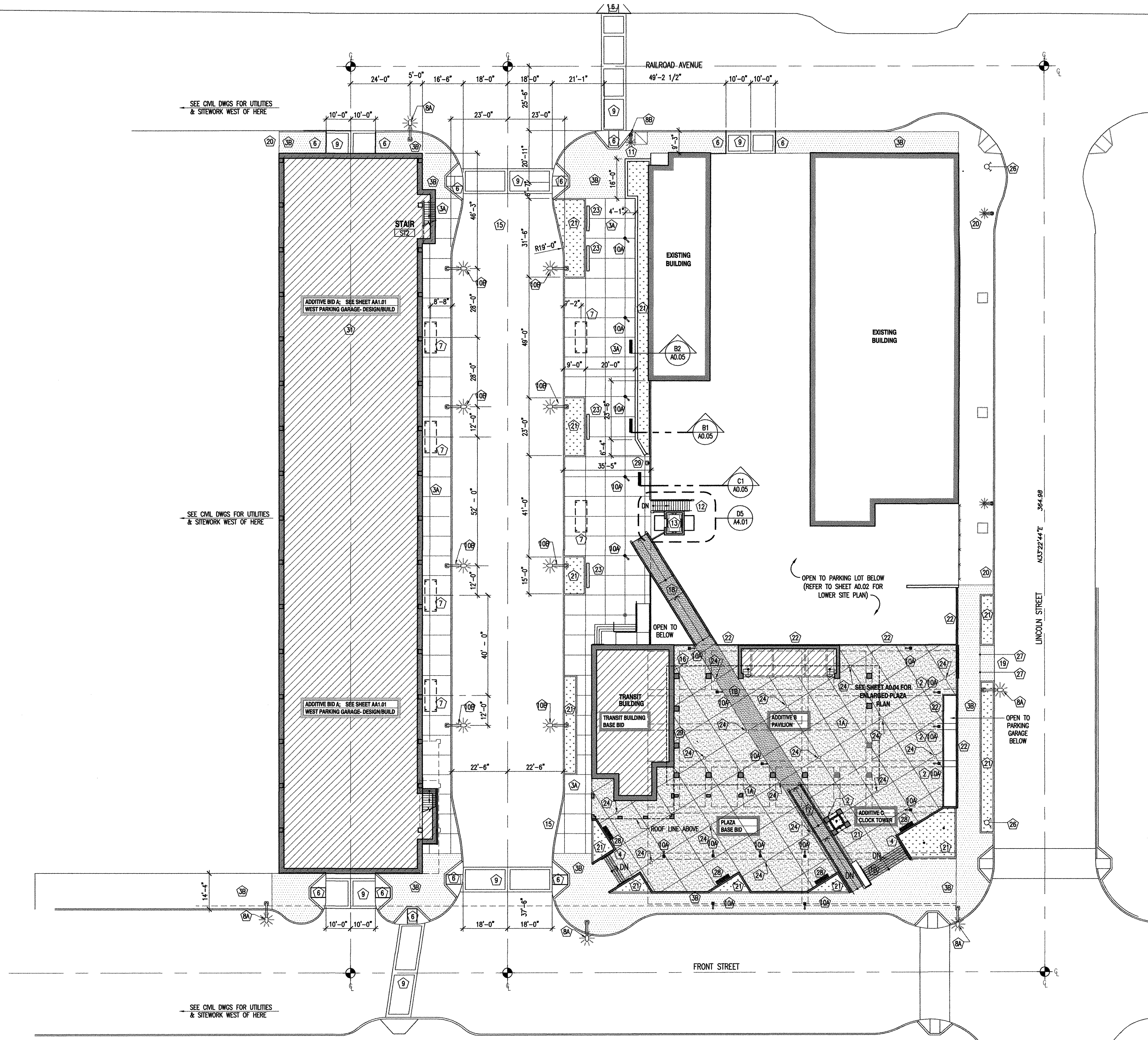
UPPER SITE PLAN SCALE: 1" = 20'-0"
